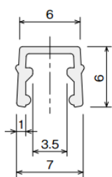
Slot Cover20
