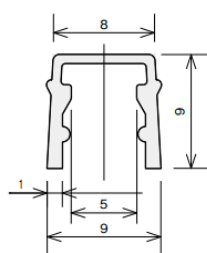
Slot Cover30
